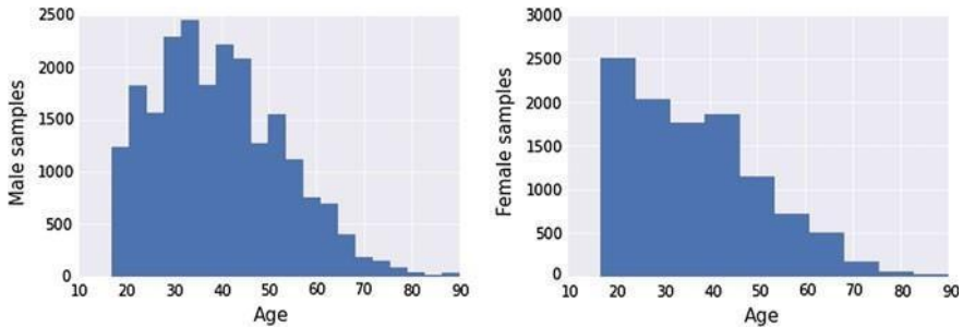
Fig. 3.1 Histogram of the age of working men ( left ) and women ( right )
